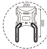
VESA 200x300
